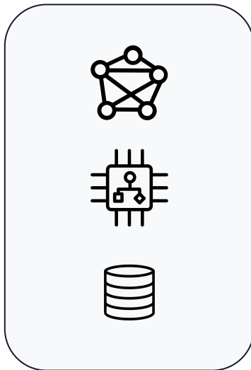
Virtual Machines
